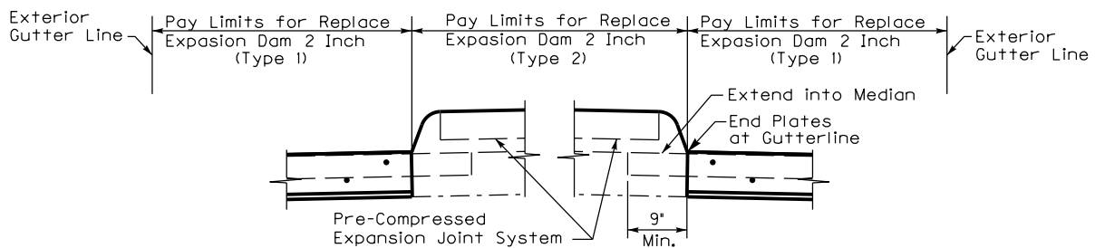
TRANSVERSE SECTION THROUGH MEDIAN Expansion Joint Replace 2" (See Standard Drawing BJE-001, BJE-003 & BJE-005 CE).
