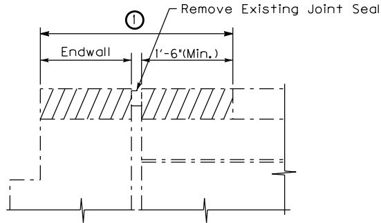
LONGITUDINAL SECTION THROUGH MEDIAN (Existing)
