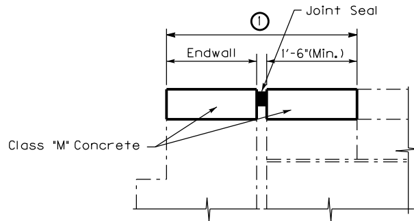
LONGITUDINAL SECTION THROUGH MEDIAN (Proposed)
